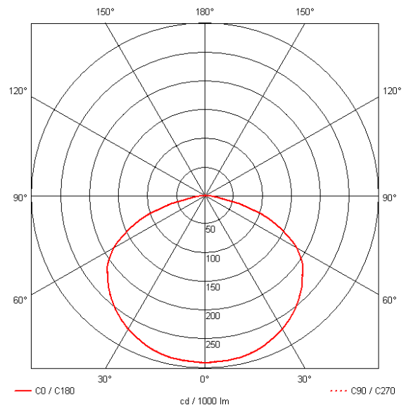
cd/1000 lm
