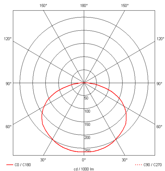
cd/1000 lm
